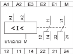
Wiring Diagram
