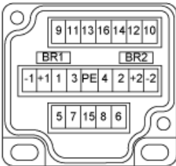
Connection Terminals
