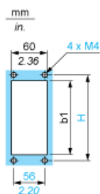
Panel cut-out
